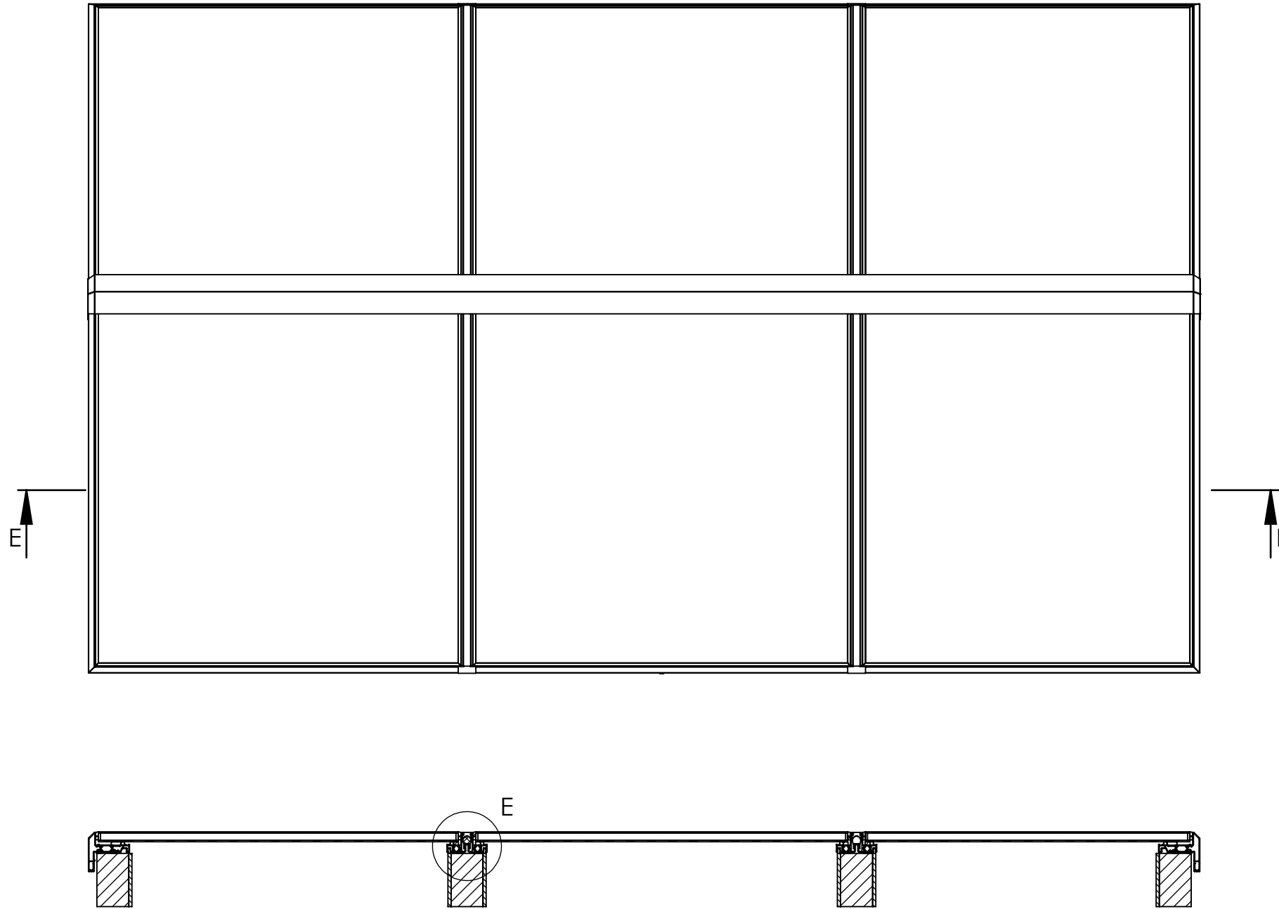
SECTION E-E
