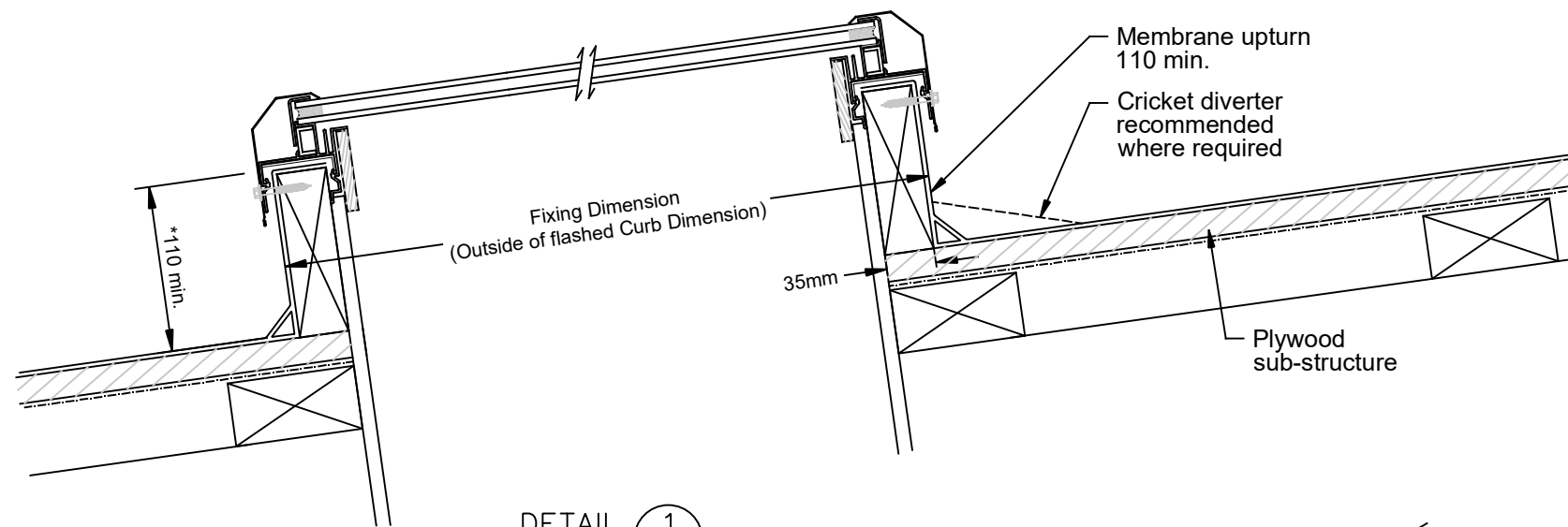
DETAIL 1
